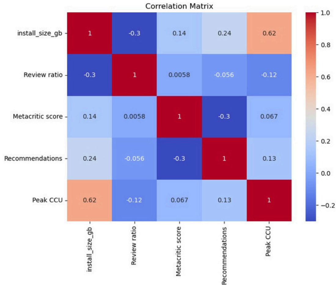
Figure 4. Correlation Matrix.
